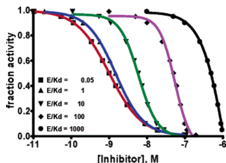
Figure 2. Dose-response curves predicted by the stoichiometric model for a 1 nM inhibitor measured at increasing enzyme concentrations: 50 pM enzyme (red, 0.05K_d ), 1 nM enzyme (blue, K_d ), 10 nM enzyme (green, 10K_d ), 100 nM enzyme (purple, 100K_d ), 1 \mu M enzyme (black, 1000K_d ). All curves were from GraphPad Prism using a sigmoidal dose-response curve model with variable slope. A general version of this figure may be found in ref 13.
