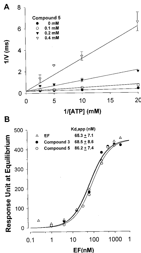
FIG. 6. Characterization of compounds 3 and 5 on the mechanism of inhibition. A, kinetic properties in the inhibition of EF by compound 5 . The adenylyl cyclase assay was done in the presence of 16 \mu M EF3, 1 \mu M CaM, 1 \mu M free Ca^{2+} , and the indicated concentrations of compounds. The V_{max} , K_m , and K_i values were estimated to be 5 ms^{-1} , 50 \mu M , and 20 \mu M , respectively. B, the effect of compounds 3 and 5 on the binding of EF to CaM. Apparent K_d was calculated using a simple one-to-one-binding model: R_{eq} = R_{Max} \times ([EF]/([EF] + K_d^{app})) where, R_{eq} , R_{Max} , and K_d^{app} are responses at equilibrium, maximum response at excess EF, and apparent dissociation constant, respectively. The SPR spectroscopy was performed in the presence of Me 2 SO alone (open triangles), 500 \mu M compound 3 (filled circles), and 500 \mu M compound 5 (open circles). Mean \pm S.E. are representative of at least two experiments.
