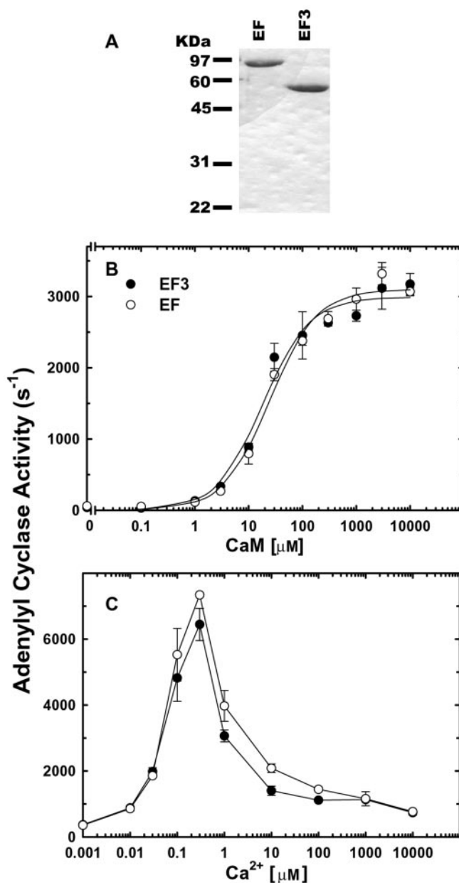
FIG. 1. Effect of CaM and calcium ion on adenylyl cyclase activity of EF, a full-size EF, and EF3, a catalytic domain of EF. A, purified EF and EF3. 1 \mu\text{g} of purified EF and EF3 were run on an SDS-polyacrylamide gel and stained by Coomassie Blue. B, adenylyl cyclase assays were performed with 0.78 nM EF (open circles) and 0.85 nM EF3 (filled circles) in the presence of 1.0 \mu\text{M} free \text{Ca}^{2+} . C, adenylyl cyclase activities were measured with 0.52 nM EF (open circles) and 0.56 nM EF3 (filled circles) in the presence of 10 \mu\text{M} CaM. Mean \pm S.E. are representative of at least two experiments.
