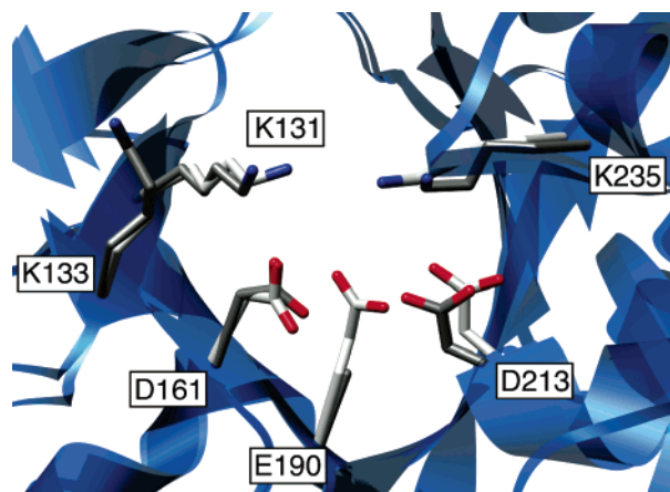
FIGURE 2: Structural superposition of the OSBS wild-type structure (light gray) and the E190A mutant structure (dark gray).
