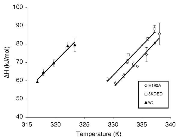
FIGURE 3: van't Hoff plots for wild-type OSBS (▲), E190A (◇), and 3KDED (□).
