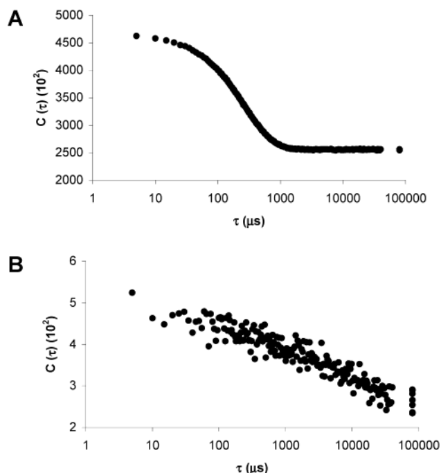
Figure 7. Representative autocorrelation functions from DLS on aggregate-forming inhibitors with and without Triton X-100: (A) 10 \mu M I4PTH alone; (B) 10 \mu M I4PTH with 0.01% Triton X-100.
