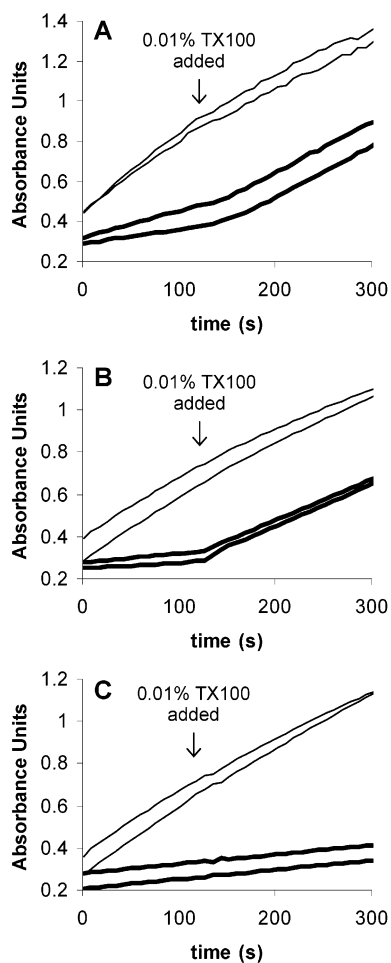
Figure 5. Effect of 0.01% Triton X-100 added during a \beta -lactamase inhibition assay. (A) Inhibitor is 10 \mu M I4PTH. (B) Inhibitor is 5 \mu M rottlerin. (C) Inhibitor is 0.6 \mu M BZBTH2B, a specific \beta -lactamase inhibitor. 21 In all panels, thick lines (—) denote reactions containing inhibitor and thin lines (—) denote reactions containing DMSO control. TX100 is Triton X-100.
