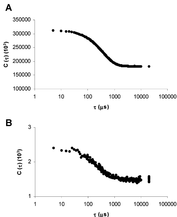
Figure 1. Representative autocorrelation functions from DLS before and after centrifugation of promiscuous inhibitors. (A) Autocorrelation function of 100 \mu\text{M} I4PTH before centrifugation. The average intensity was 366 kcps (kilocounts per second), and the \text{IC}_{50} vs \beta -lactamase was 3 \mu\text{M} . (B) Autocorrelation function of 100 \mu\text{M} I4PTH after centrifugation. The average intensity was 1 kcps, and the \text{IC}_{50} vs \beta -lactamase was 70 \mu\text{M} . Laser power and integration times were comparable for all DLS experiments.
