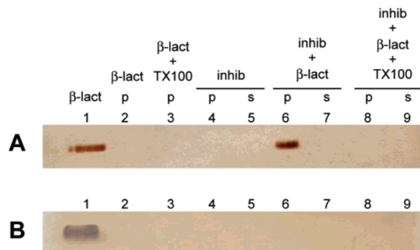
Figure 2. SDS-PAGE and silver-stain analysis of supernatants and pellets from centrifugation of \beta -lactamase in the presence or absence of inhibitor with and without Triton X-100. (A) The inhibitor is tetraiodophenolphthalein (I4PTH), a promiscuous, aggregate-forming compound. 17 (B) The inhibitor is 1-(2-thienylacetyl-amino)-1-(3-carboxyphenyl)methylboronic acid, a specific, nonaggregating inhibitor of \beta -lactamase. 19 For both gels, lane 1 is 3000 ng of \beta -lactamase loaded directly onto the gel, lane 2 is the pellet from centrifugation of \beta -lactamase alone, lane 3 is the pellet from centrifugation of \beta -lactamase with 0.01% Triton X-100, lanes 4 and 5 are the pellet and supernatant from centrifugation of 100 \mu\text{M} inhibitor alone, lanes 6 and 7 are the pellet and supernatant from centrifugation of 100 \mu\text{M} inhibitor with \beta -lactamase, and lanes 8 and 9 are the pellet and supernatant from centrifugation of 100 \mu\text{M} inhibitor with \beta -lactamase and 0.01% Triton X-100. A 3000 ng sample of \beta -lactamase was used for each centrifugation experiment. Abbreviations are the following: s, supernatant; p, pellet; \beta -lact, \beta -lactamase; TX100, Triton X-100; inhib, inhibitor.
