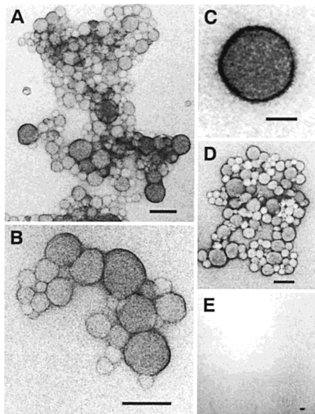
Figure 2. Compounds visualized by transmission electron microscopy: (A–C) 100 \mu\text{M} tetraiodophenolphthalein in 20 mM Tris; (D) 50 \mu\text{M} Congo Red in 20 mM Tris; (E) 625 \mu\text{M} ANS in 20 mM Tris. Bar = 100 nm.
